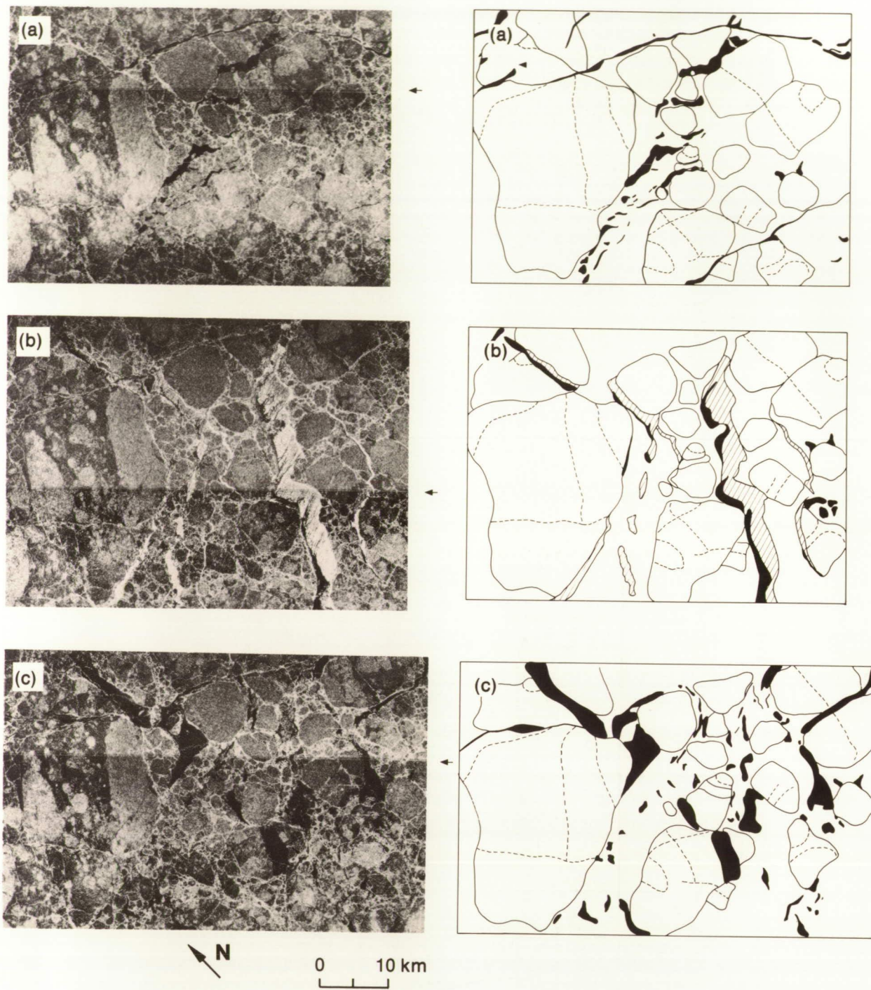
Figure 8. Enlargements of three Seasat images taken over a 6-day period in Melville Sound, Canada. The corresponding sketch maps indicate major floes (solid lines) with some distinguishing features (dashed lines), leads and/or new ice (dark zones), and grease ice "tadpoles" (stripped zones). Arrows indicate adjoining swaths: (a) Rev. 1365, September 30, 1978; (b) Rev. 1408, October 3, 1978; (c) Rev. 1451, October 6, 1978.
